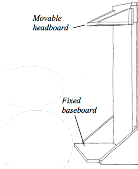
Figure 3.3: Height board mounted upright
