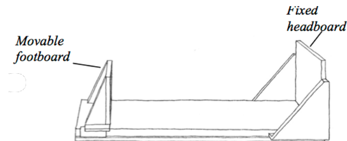
Figure 3.2: Length board flat on a table surface
